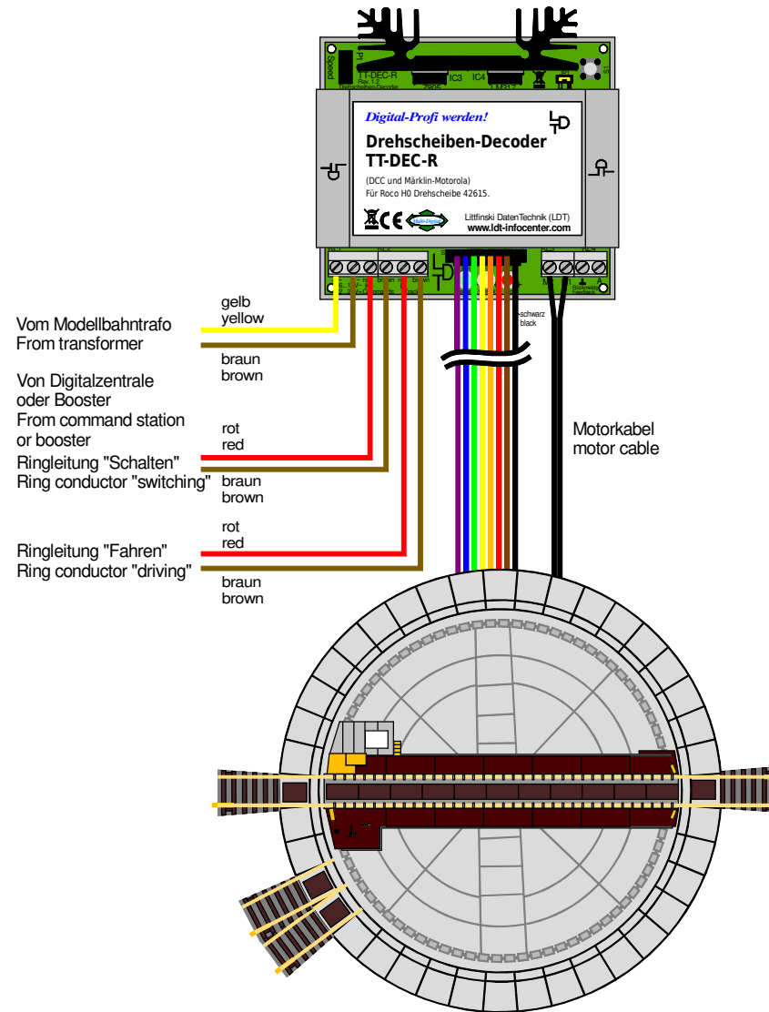
Roco Drehscheibe 42615 alte Variante Roco Turntable 42615 old version
